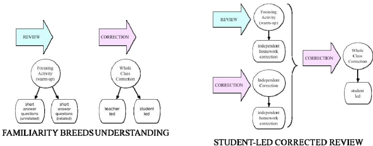
Figure 2. Iconic Sequences
